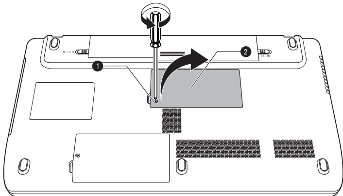
Figure 3-9 Removing the memory module cover (Satellite L770/L775/L770D/L775D/satellite Pro L770/L775/L770D/L775D)
